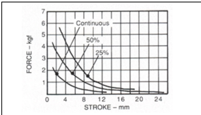
DC OPERATED (Typical)
