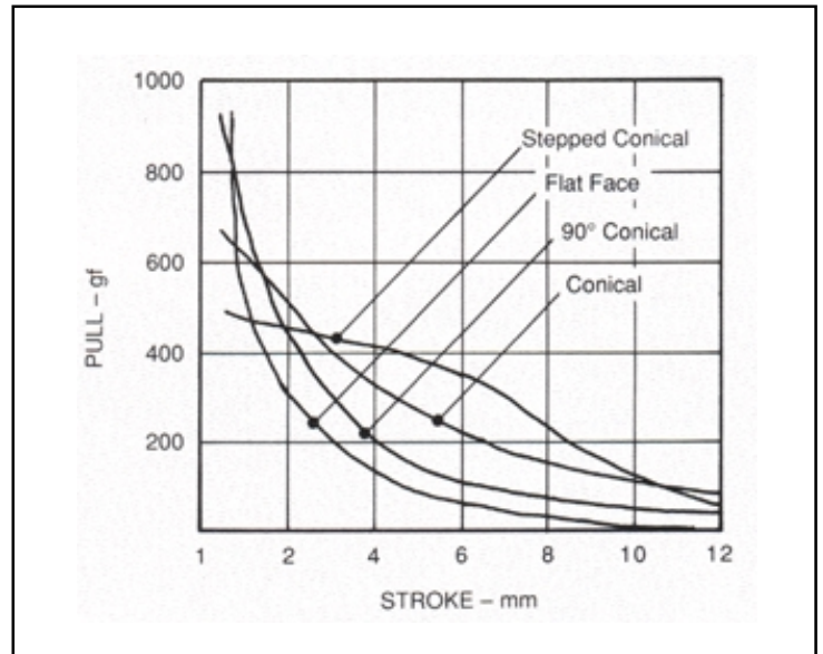
Plunger end styles Pull/Stroke comparison
