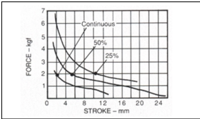
AC OPERATED (Typical)
