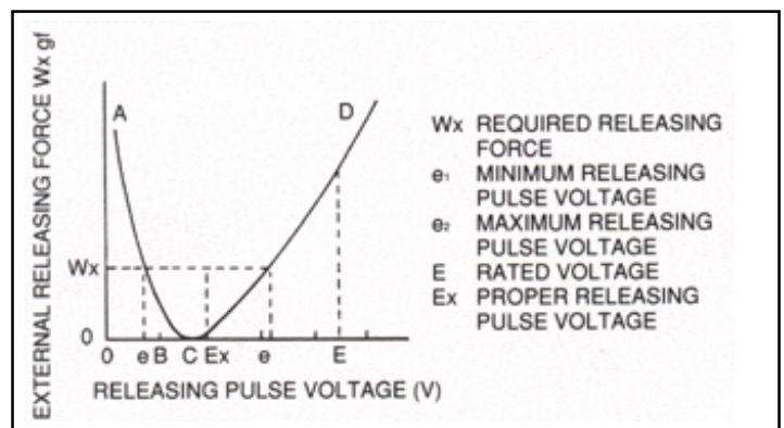
Relationship between releasing force and releasing pulse voltage
